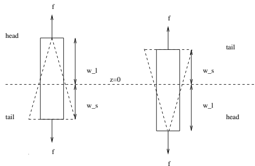
Fig. 3. The asymmetric dipole model of the pumps described in the Appendix. The centers of mass of the pumps are displaced above or below the bilayer midpoint. The distance of the furthest force-centre from z = 0 is w_l and the distance of the nearest force-centre from z = 0 is w_s .
