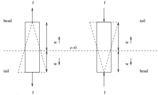
Fig. 2. The asymmetric dipole model used to describe the activity of the proteins. The force-centres are placed at distances w^\uparrow and w^\downarrow from the bilayer midpoint. The centers of mass of the pumps are displaced above the bilayer midpoint. The superposed “up” and “down” triangles indicate the underlying shape asymmetry of the two different kinds of pumps.
